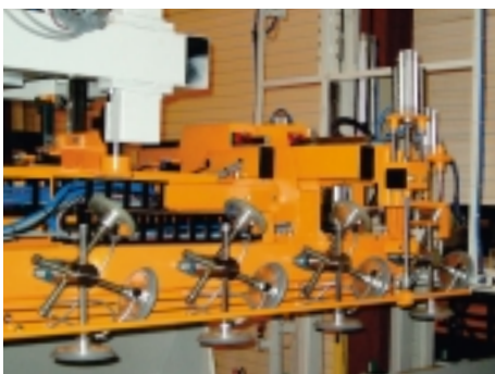
fully automatic change of suction cups
